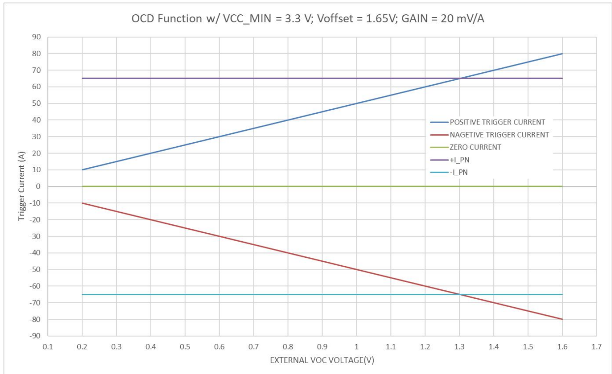
OCD function for STK-616K-65FC
